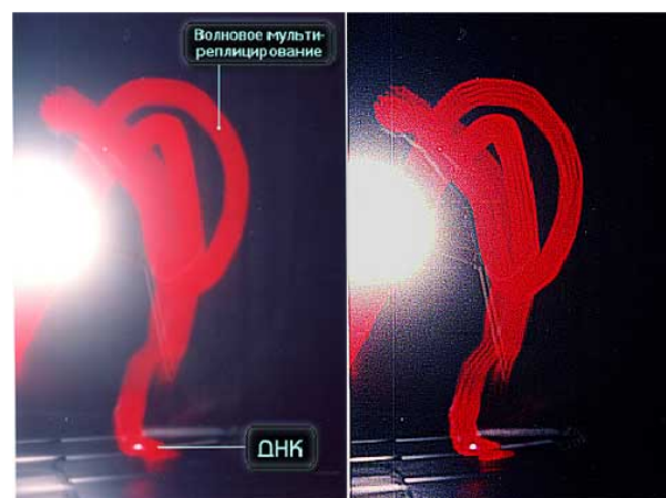
Figure 3: The picture shows the discrete replica like structure of the band like image obtained by method I and interpreted by experimenters as replica image of DNA sample. To the left image is the original image and to the right the contrasted one.
