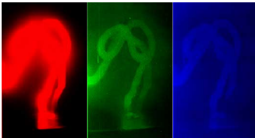
Figure 5: Long living DNA wave replica from the experiment in Fig. 3 (referred to as phantom image as opposed to the image seen during irradiation) subsequent to switching off of the initiating electromagnetic fields/frequencies sources.
