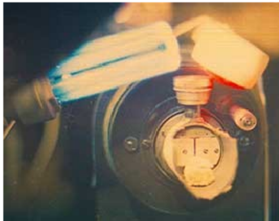
Figure 7: a) The moment of mechanical external interference (touch, which could have also biological effect) with DNA sample. The second method of elicitation of DNA wave replicas. b) Shift to the left of the wave replicas immediately after the interference. It is also commonly noticed that there is a sharp distinction of the shot from others by brightness and color scheme, which is unrelated to the working of the camera.
